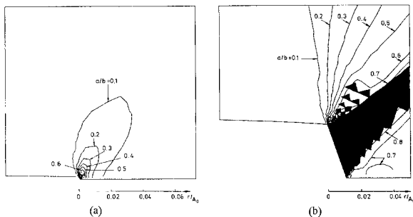
Fig. 2: Distributions of creep damage ahead of a crack-tip. Continuous cavity nucleation, no grain boundary sliding, and C = 40 . (a) t/t_f^0 = 0.064 . (b) t/t_f^0 = 0.686 . (From [18]).
