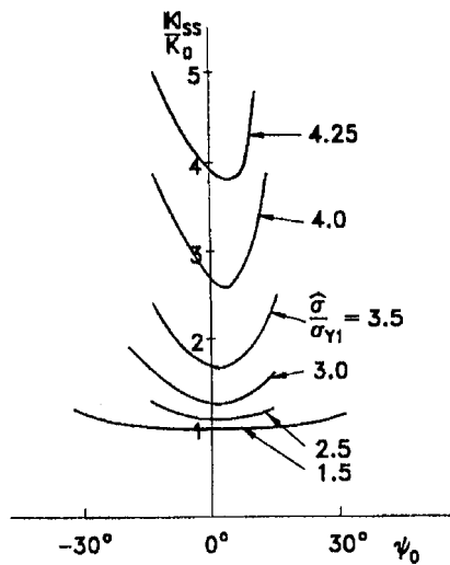
Fig. 3: Steady-state interface toughness as a function of the local mixity measure \psi_0 , for \sigma_{y1}/E_1 = 0.003 and \sigma_{y2} \approx \infty , considering different values of \hat{\sigma}/\sigma_{y1} , E_2/E_1 = 2 . (From [23]).
