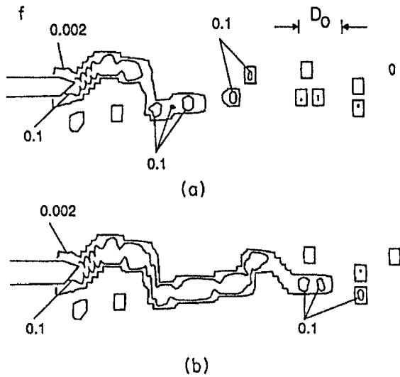
Fig. 1: Crack growth indicated by contours of constant void volume fraction, f , for random distribution of larger particles. (a) t = 1.5 \mu s , \Delta a = 0.09 \text{ mm} ; (b) t = 1.6 \mu s , \Delta a = 0.27 \text{ mm} . (From [9]).
