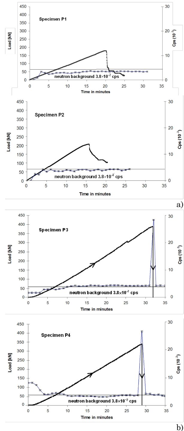
Fig. 1 – (a) Load vs. time and cps curves for test specimens P1 and P2 in Carrara marble, and (b) for test specimens P3 and P4 in Luserna granite
