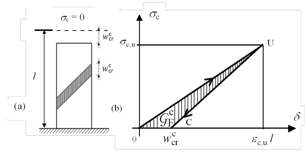
Fig. 3 – Catastrophic behaviour in a solid specimen during compression. (a) Conditions of complete interpenetration and critical value of the interpenetration length w_{\text{cr}}^c . (b) Stress vs. displacement response; \sigma_{c,u} = ultimate compression strength; \epsilon_{c,u} = ultimate compression strain; \delta = \epsilon_{c,u} l = ultimate displacement, G_F^c = crushing energy
