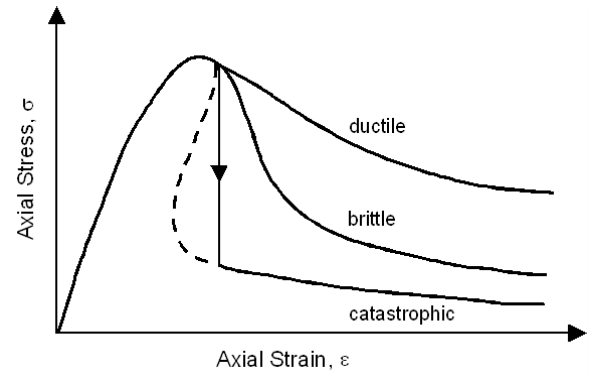
Fig. 2 – Ductile, brittle, and catastrophic behaviour
